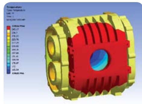
Figure 2 – With FEA thermal analysis, a good design was made great.
