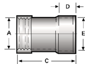
Female Reducing Adapter Expanded
