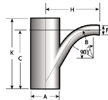
90° TY (straight ends)
