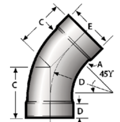
45° Short Radius Elbow
