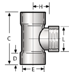
Adapter Tee
